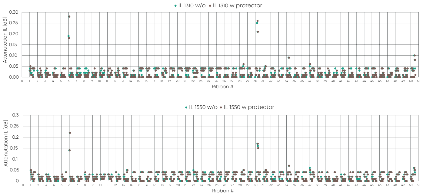
Figure 4: Scatter plot of the insertion loss of the 50 ribbons (600 measurements each) without (w/o, green) and with (w, brown) protector measured at 1310 nm (upper panel) and 1550 nm (lower panel), respectively.
