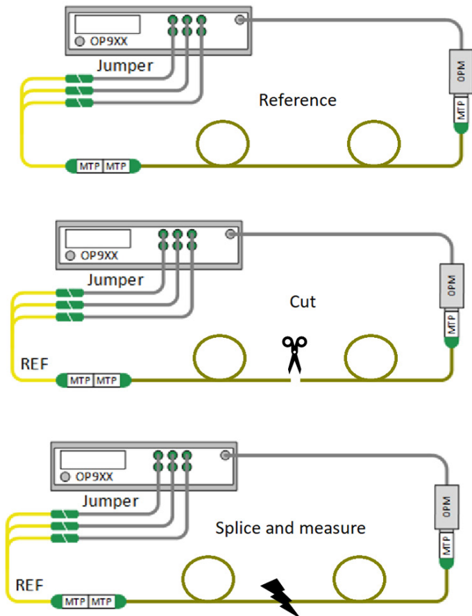
Figure 2: Measurement setup. 10 m of a flexible ribbon cable were connected with MTP to an insertion loss meter. The cable was cut in the middle, spliced and measured, the splice protector was added and the IL measured again.
