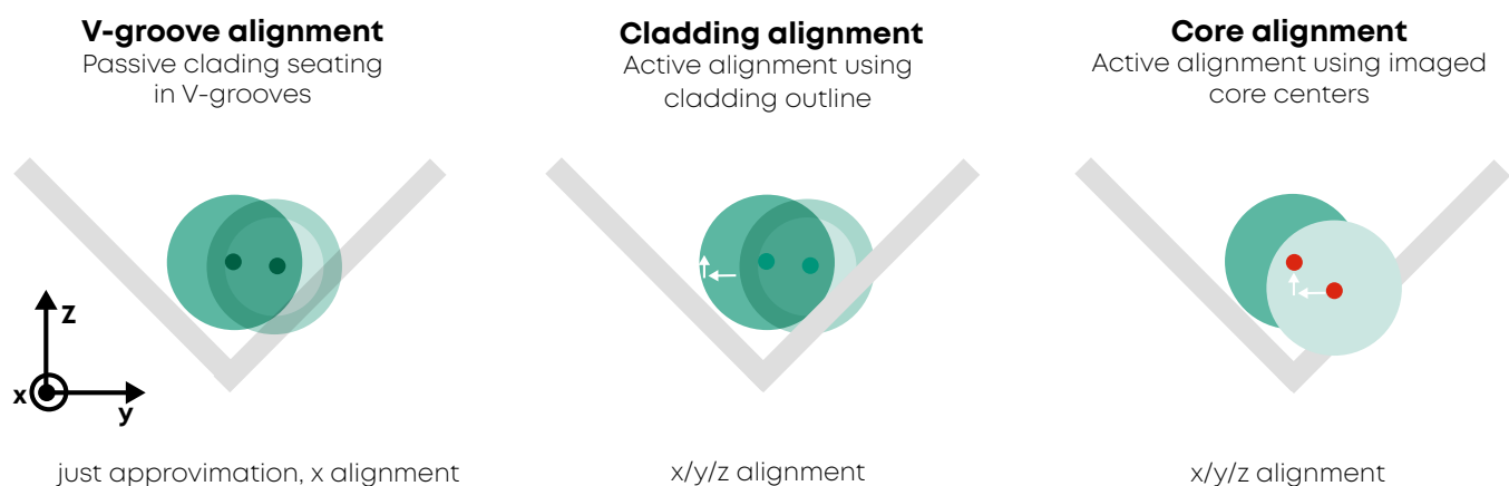
Figure 1: The three different kinds of fusion splicers characterized based on their freedom to align the fibers.
